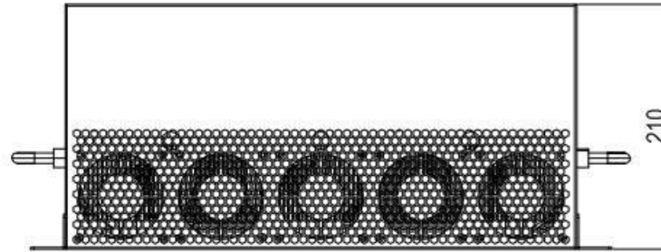
Figure 1-3 Front View
