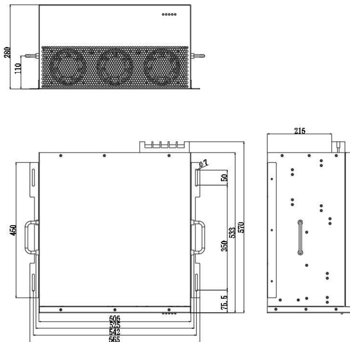
Figure 1 - 3 Overall Dimension Drawing (Unit: mm) of Rack Module(150A)
