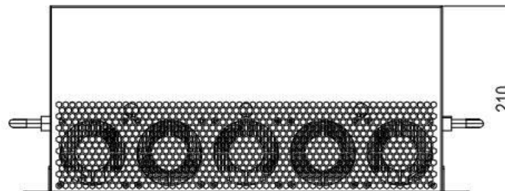
Figure 1-4 Front View
