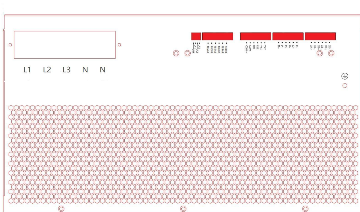
Figure 2-3 Terminal Position Diagram of Devices
