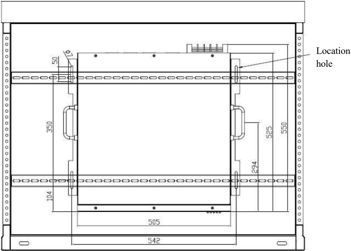
Figure 2-1 Rack Installation Diagram of Devices
