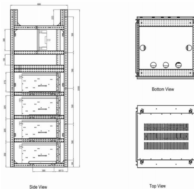
Figure 7-3 Side View, Top View and Bottom View (Unit: mm)
