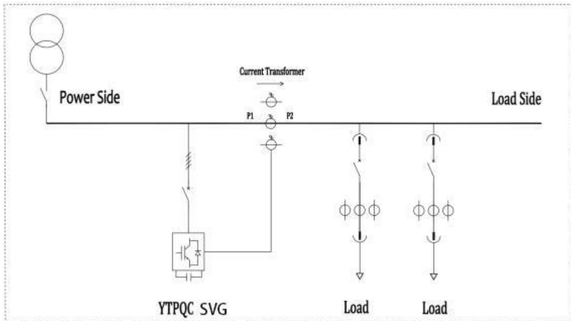
Figure 2-9 CT is at load side when single device is in operation (Preferred)
